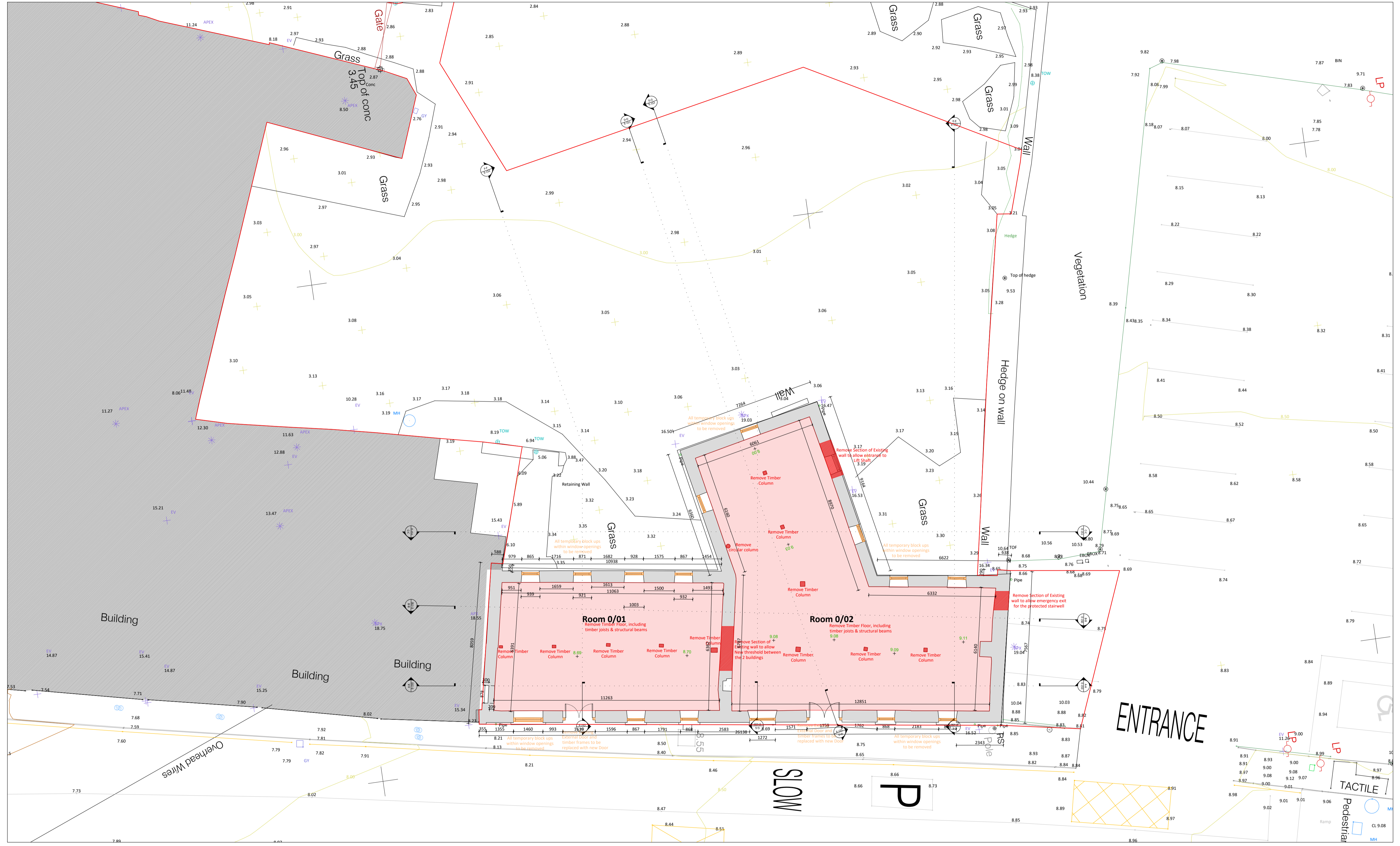
01 Level 0 (John Street) Demolition Floor Plan As Existing Scale: 1:100
